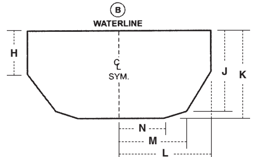
CROSS SECTION AT POINT B
