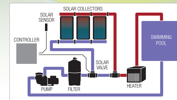
Solar pool-heating configuration
