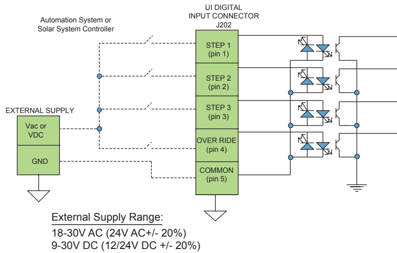
Figure 6: Wiring Diagram for Automation Control System Inputs
