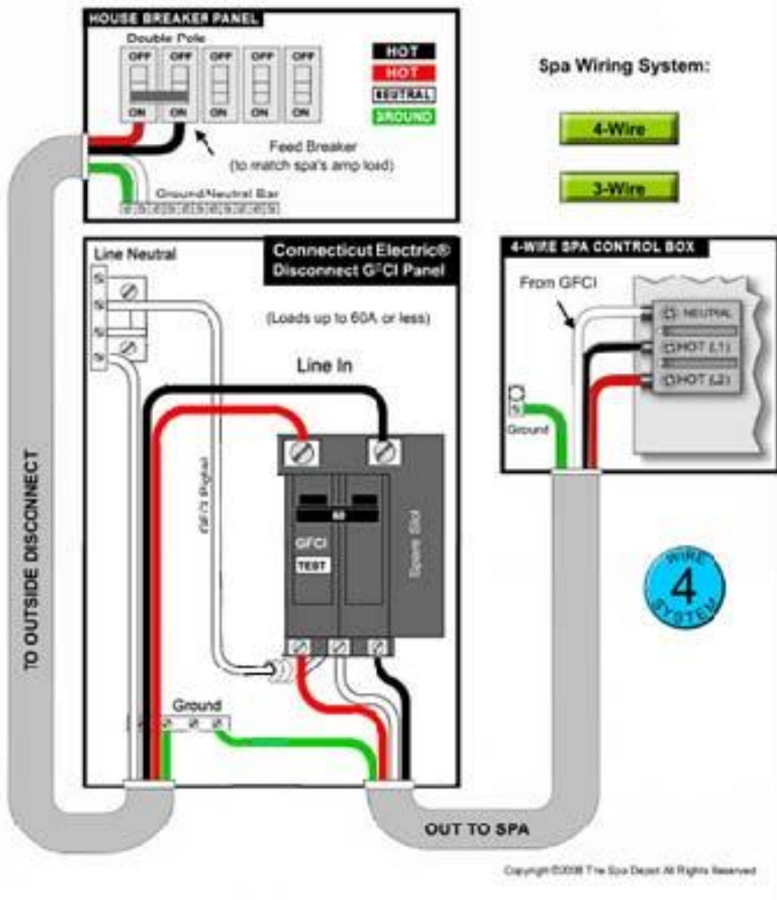
60 Hz, 240 V Residential GFCI Wiring Schematic
