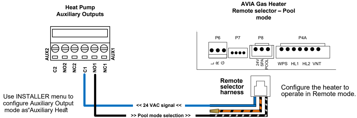
Figure 151. Example 3: Gas Heater Commanded as Auxiliary Heater
