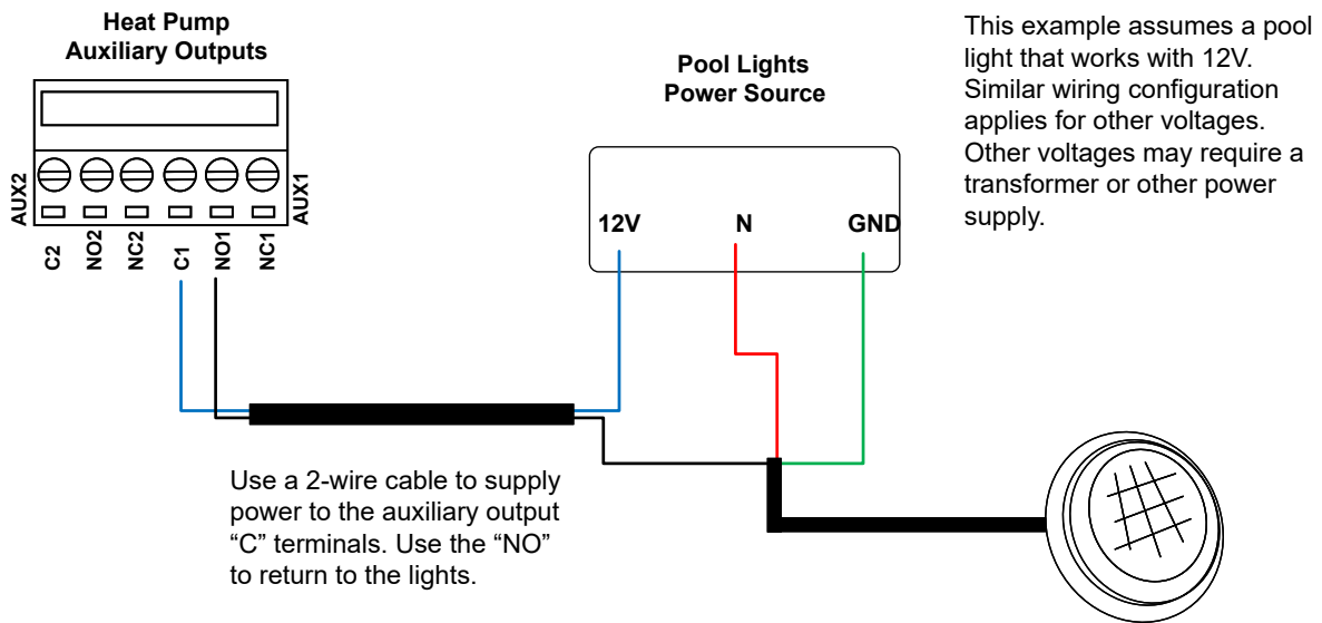
Figure 149. Example 1: Pool Light Wiring
