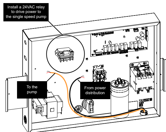
Figure 136. Install Relay in Control Box
