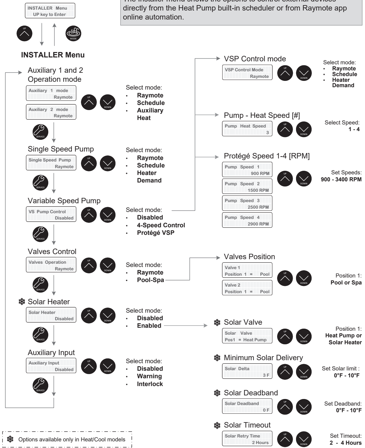
Figure 51. Installer Menu
